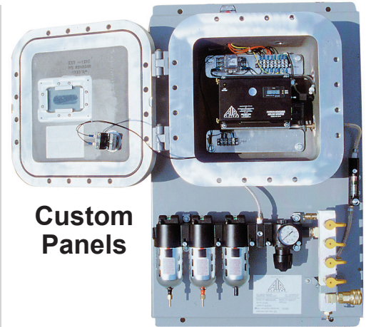
B50-COPMEX Explosion-Proof Enclosure 50 cfm Steel Panel 79 cfm flow capacity 4 couplings
